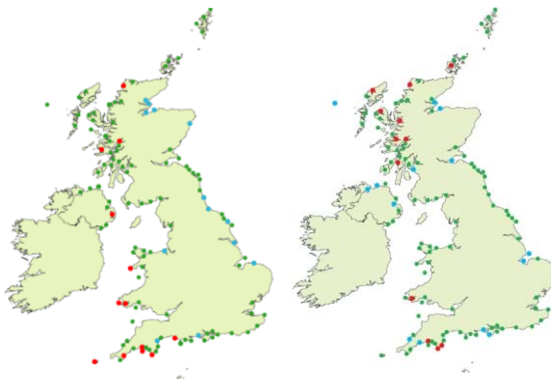
Figure 10. a) NIMF candidate species richness; and b) NIMF candidate biotope richness for coastal locations around the UK. Red dots represent 'hot' areas or higher than expected diversity, green dots represent areas of expected diversity and blue dots show areas with lower than expected diversity.
